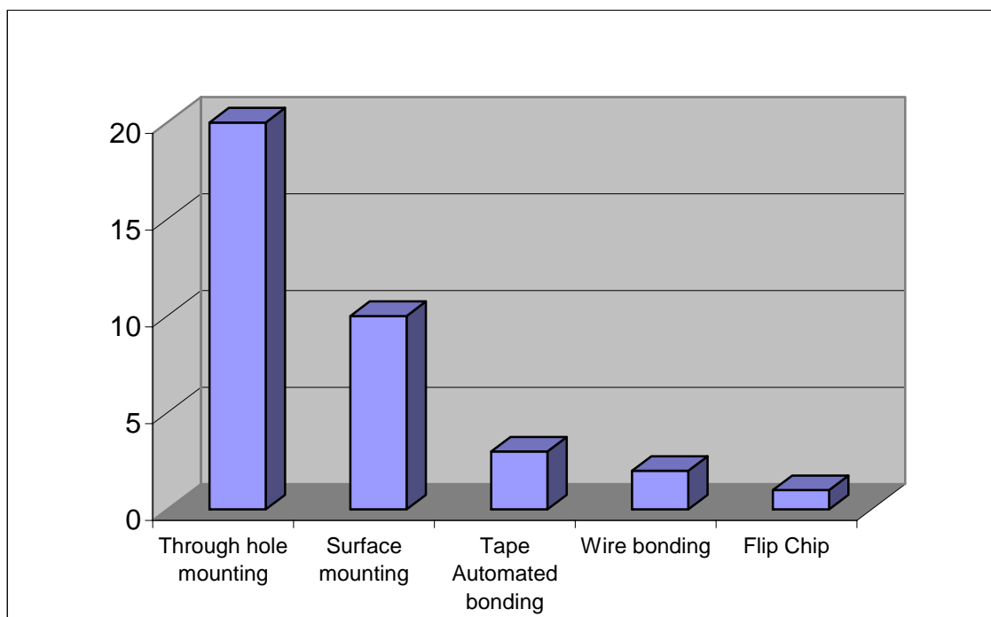
Figure 26 The relative material consumption (mg solder/bond) for different electrical interconnect technologies [Bergendahl et al. 1995]
