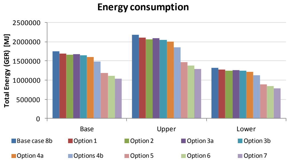
Figure 152: Sensitivity to energy consumption for Base-Case 8b's TEC
