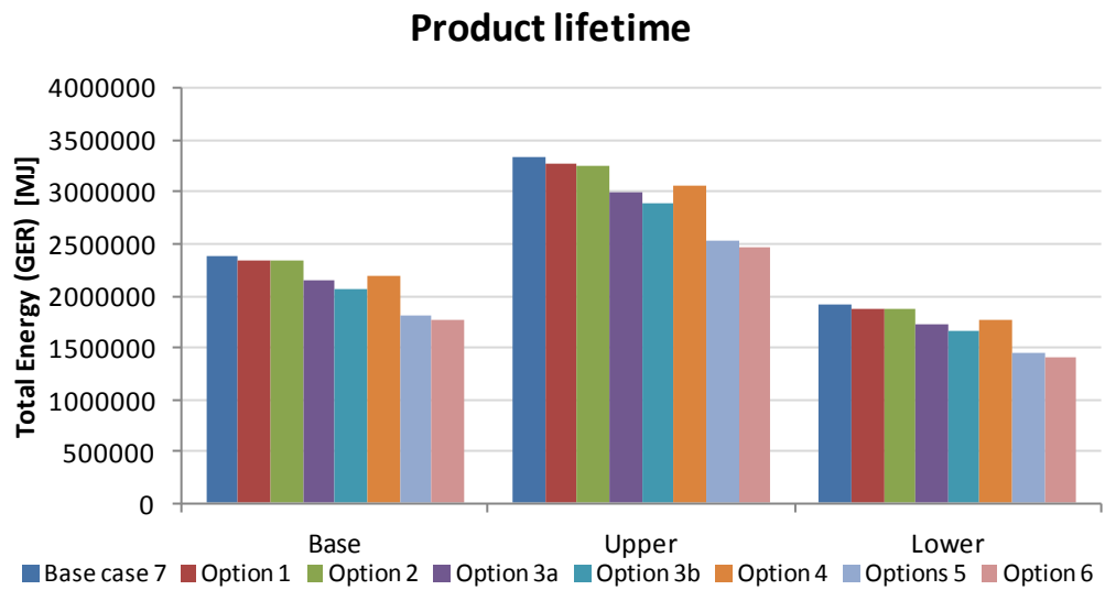
Figure 81: Sensitivity to product lifetime for Base-Case 7's TEC
