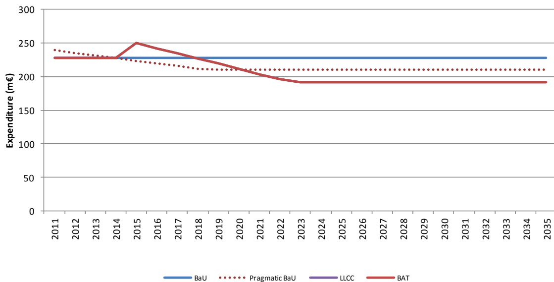
Figure 63: Comparison of the total expenditure (in million Euros) for the four scenarios over the period 2011-2035 for BC 9
