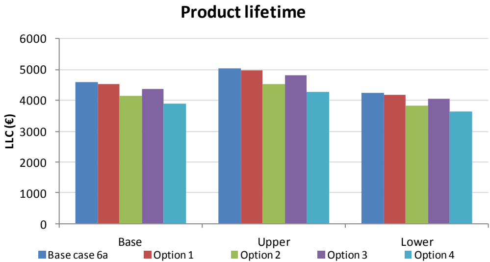
Figure 76: Sensitivity to product lifetime for Base-Case 6a’s Life Cycle Cost
