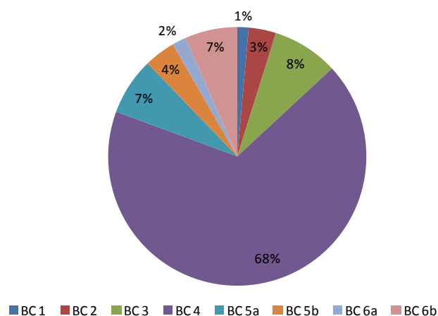
Figure 7: Residential heaters Base-Case share (in %) of total energy consumption over the period 2011-2035 in Pragmatic BaU scenario
