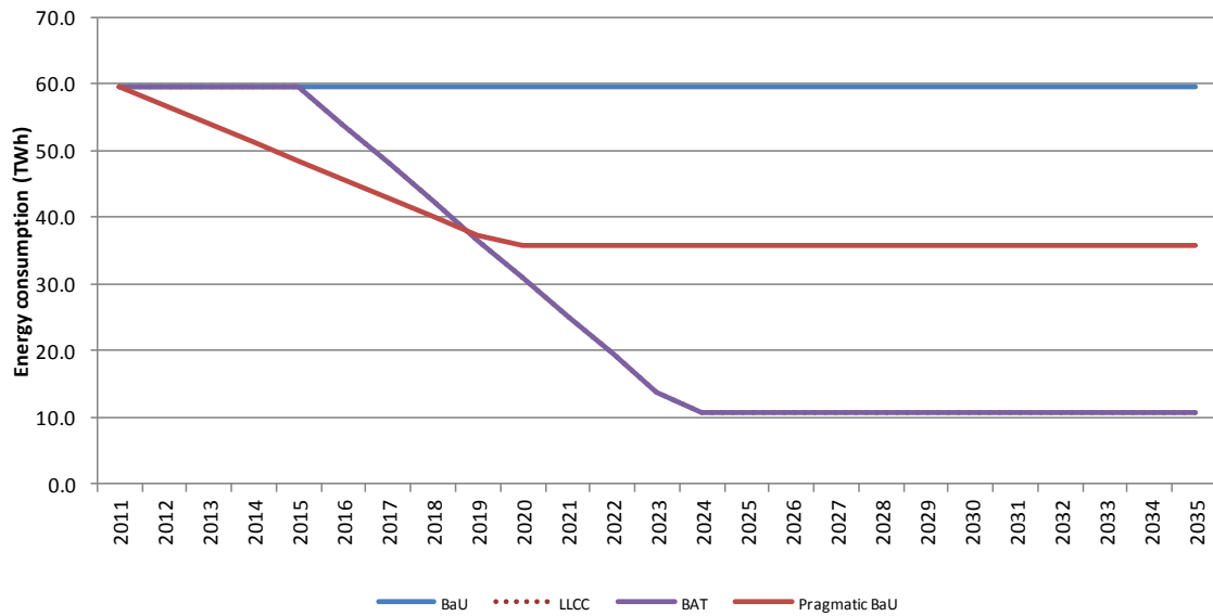
Figure 30: Comparison of the total energy consumption (in TWh) for the four scenarios over the period 2011-2035 for BC 3
