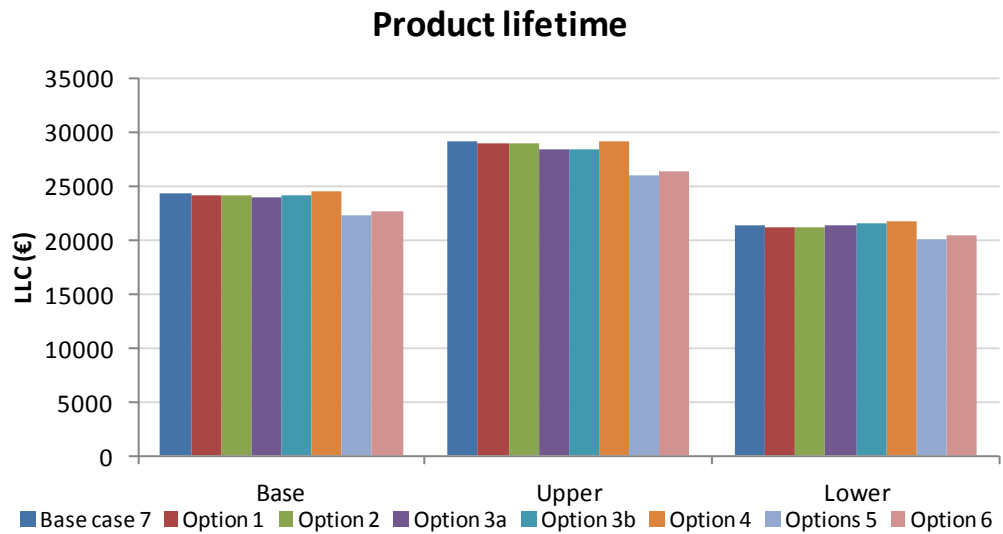
Figure 80: Sensitivity to product lifetime for Base-Case 7's Life Cycle Cost
