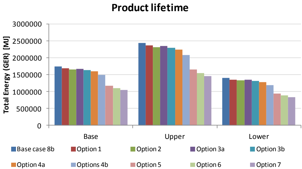
Figure 85: Sensitivity to product lifetime for Base-Case 8b's TEC
