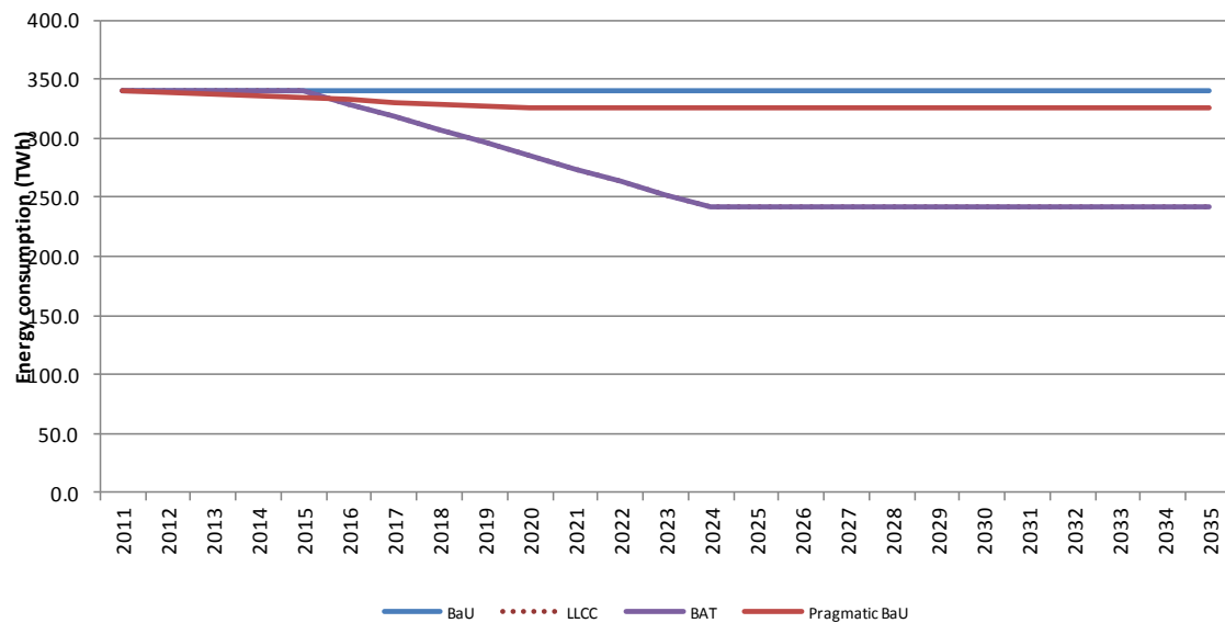
Figure 31: Comparison of the total energy consumption (in TWh) for the four scenarios over the period 2011-2035 for BC 4
