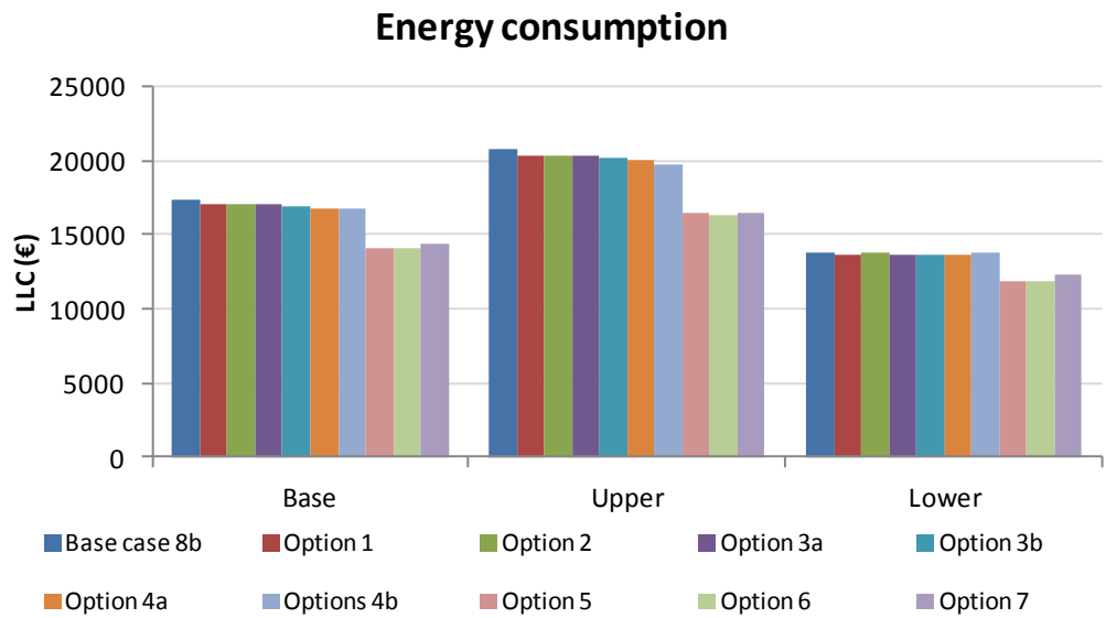
Figure 151: Sensitivity to energy consumption for Base-Case 8b's Life Cycle Cost
