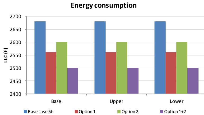
Figure 142: Sensitivity to energy consumption for Base-Case 5b's TEC
