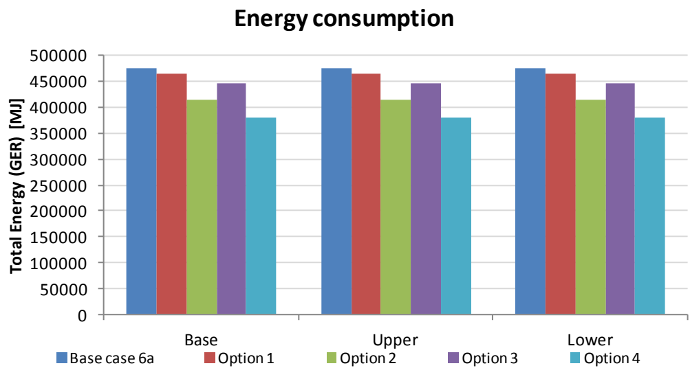
Figure 144: Sensitivity to energy consumption for Base-Case 6a’s TEC
