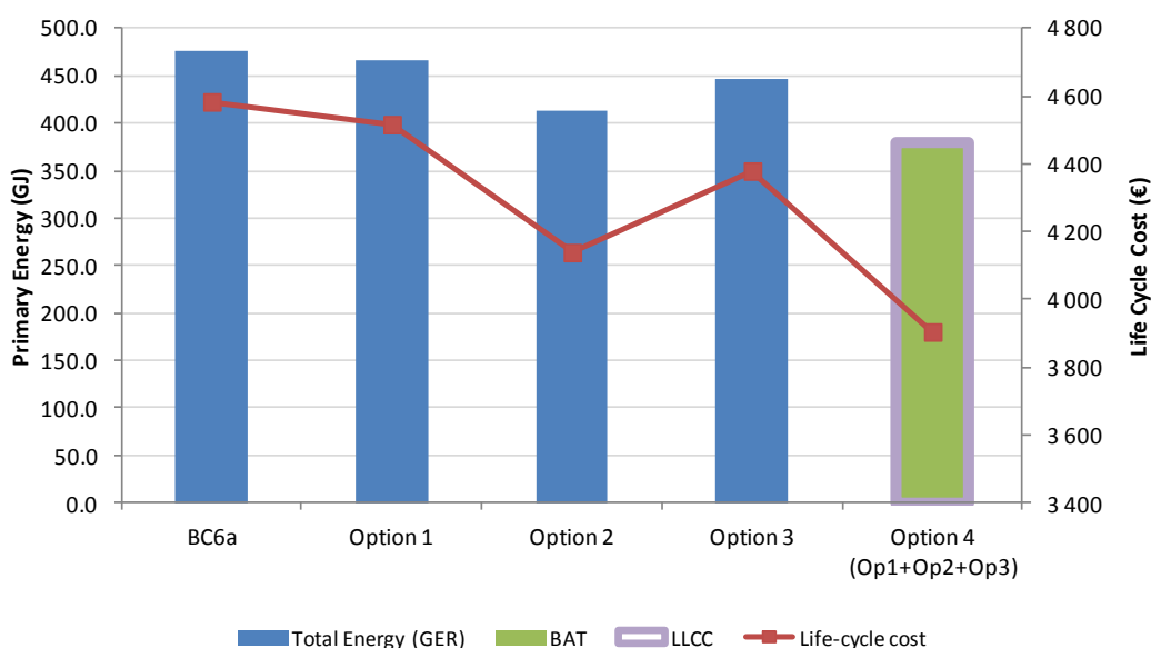
Figure 7-14: Identification of BAT option and LLCC option for BC 6a
