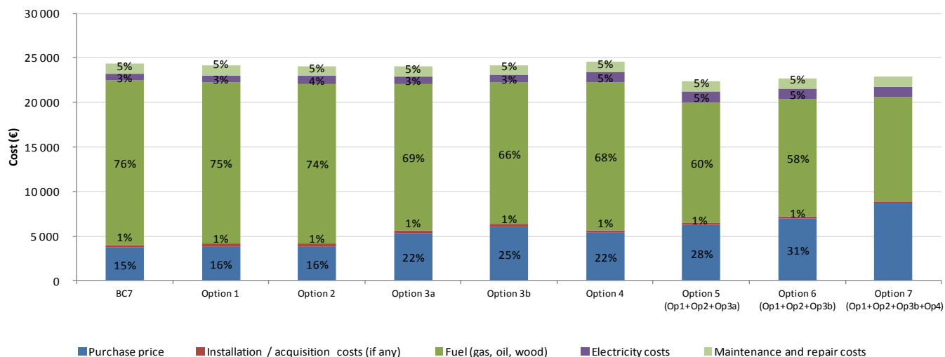
Figure 7-17: Life cycle cost of the improvement options for BC 7
